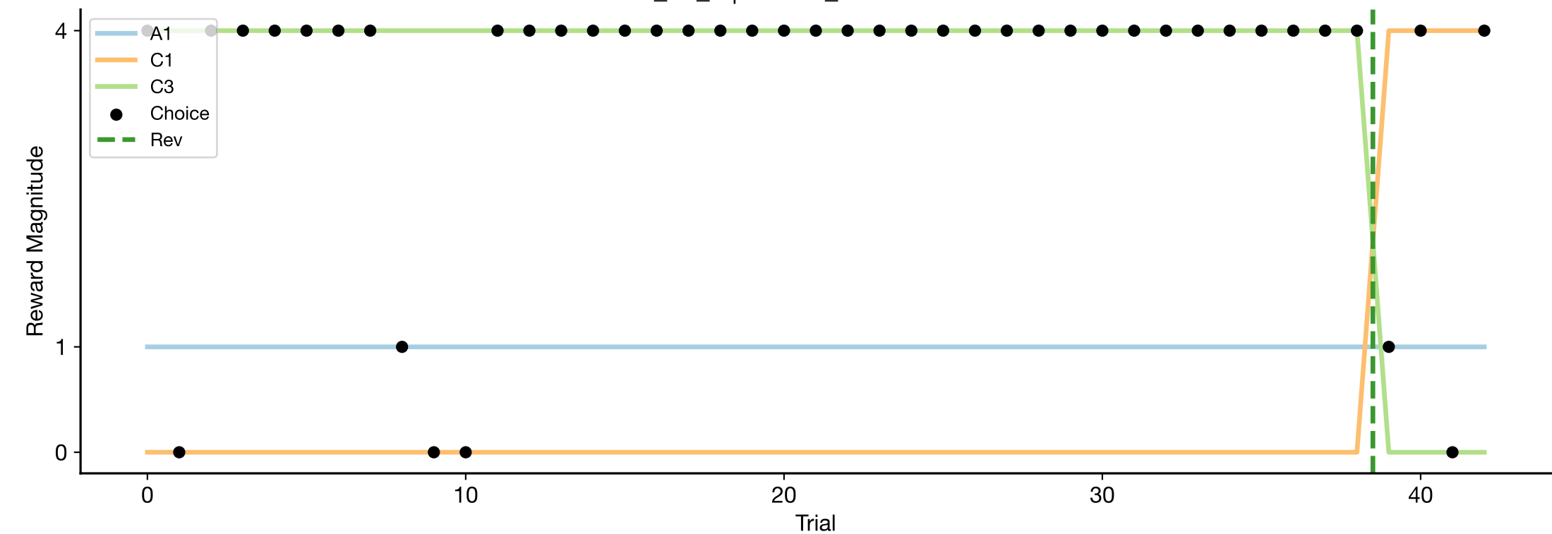
MY_71_L | ses-46_date-20260228
